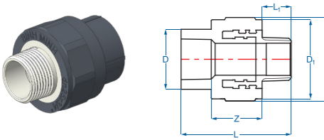
NỐI REN NGOÀI / Male thread socket
