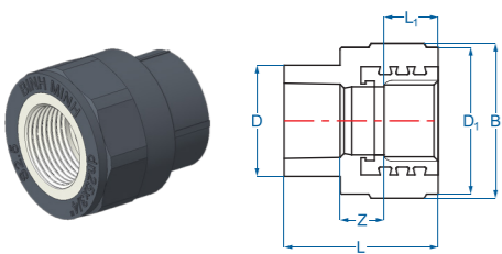
NỐI REN TRONG / Female thread socket
