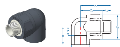
CO 90° REN NGOÀI / Male thread 90° Elbow
