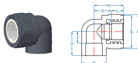
CO 90° REN TRONG / Female thread 90° Elbow
